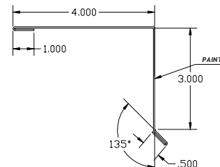
Side Rake Conc. - LSRC6
