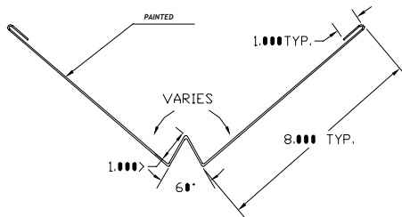
"W" Valley – LWV6—
