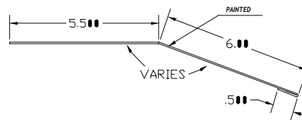
Gambrel Transition – LGT6—
